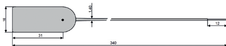
Abmessungen in mm
